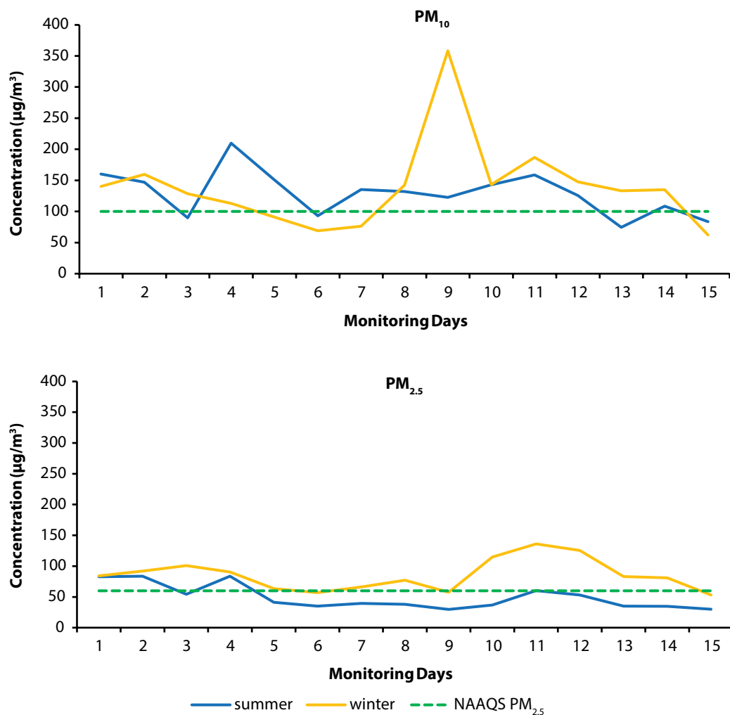
FIGURE 2.5: Variations of PM_{10} and PM_{2.5} concentrations for different seasons at residential location 1
