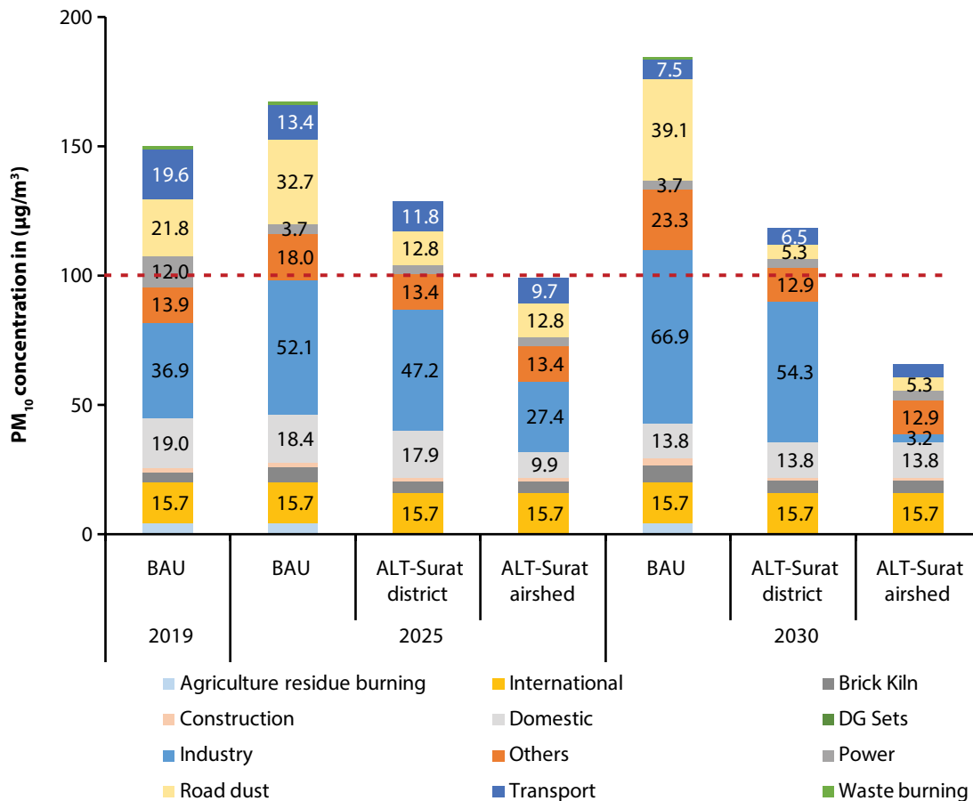
FIGURE 8.8: Winter season PM_{10} concentration in different scenario in the Surat city
