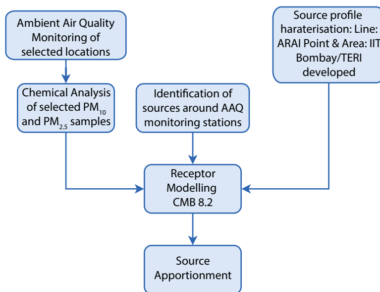
FIGURE 1.4: Approach to source apportionment using receptor model in Surat city
