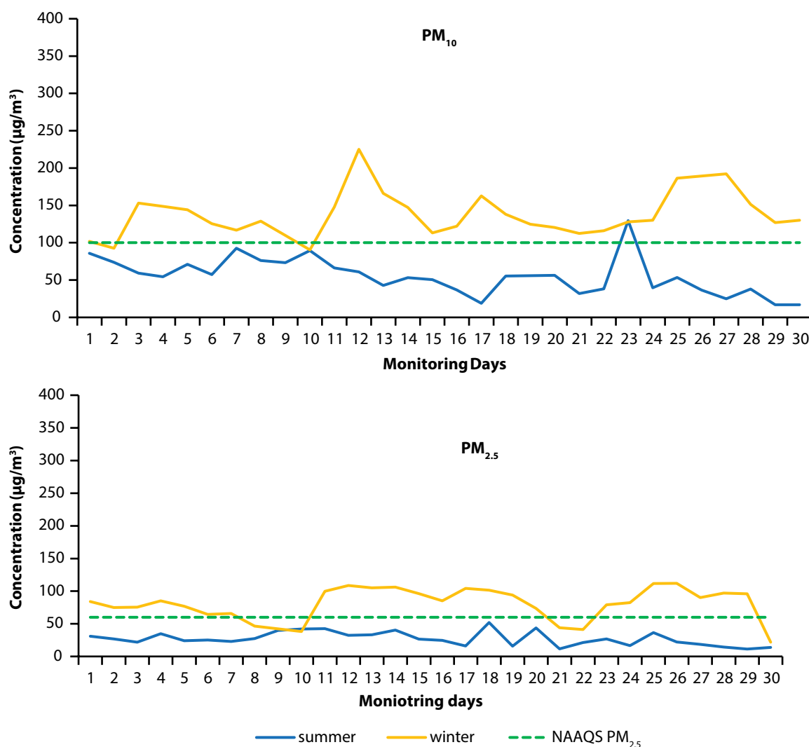
FIGURE 2.3: Trend of PM_{10} and PM_{2.5} levels for different seasons at Background location
