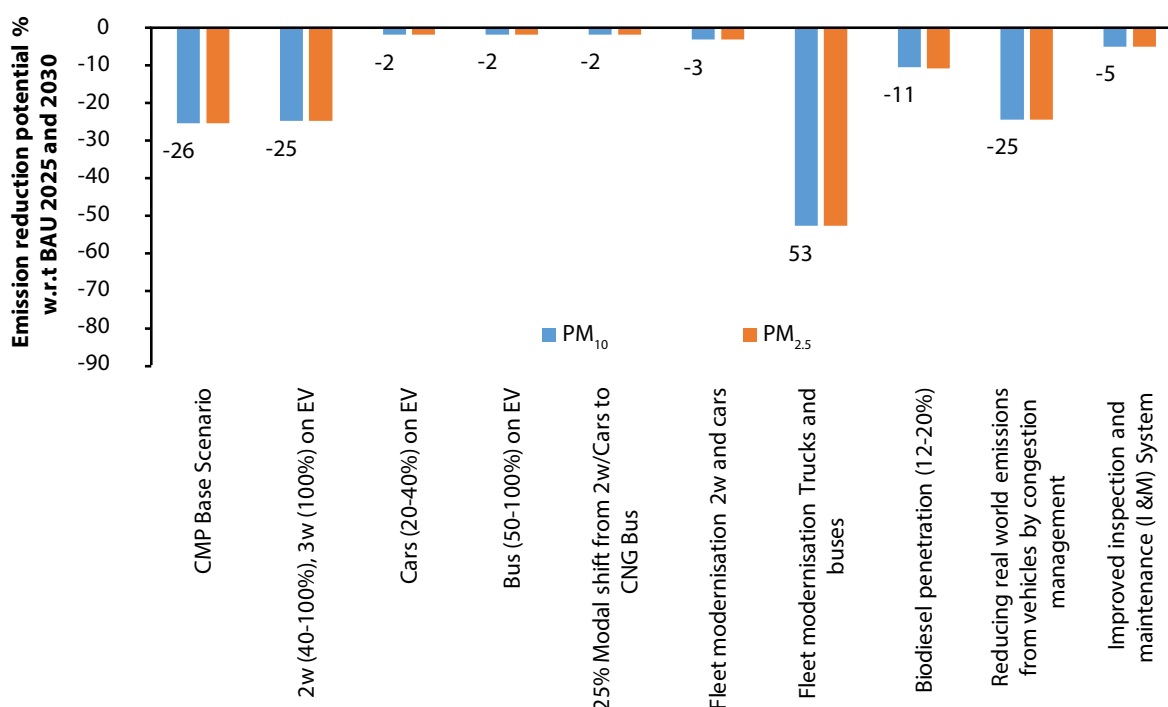
FIGURE 8.4 : PM 10 and PM 2.5 emission reduction potential of various strategies with respect to BAU 2030 transport sector emissions
