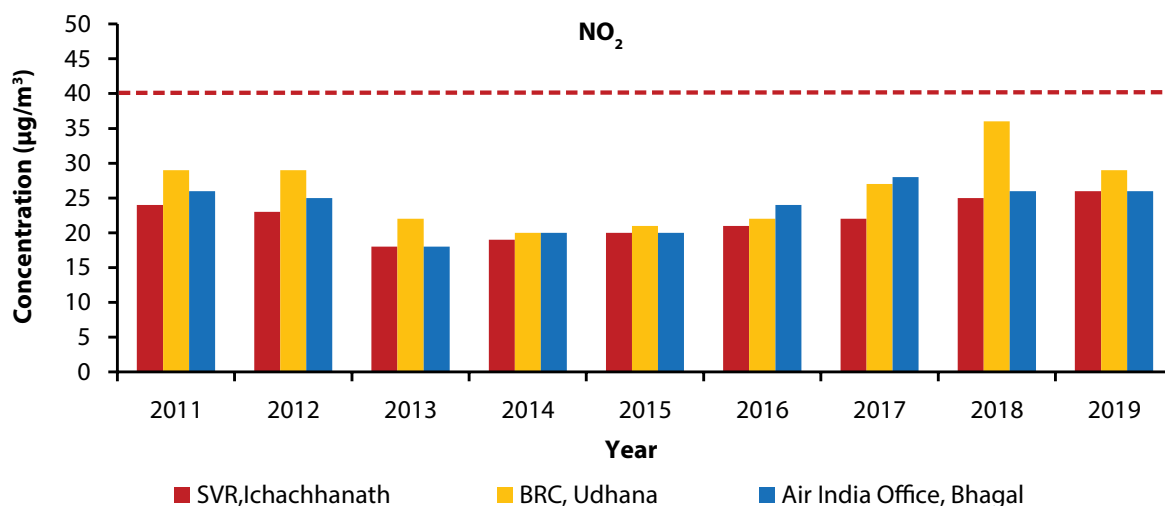
FIGURE 1.8: Annual average pollutant concentration trend during 2011-19 at different stations in Surat city
