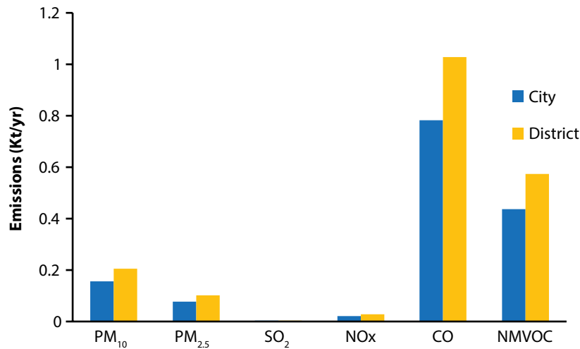
FIGURE 5.18: City and district level emissions from crematories
