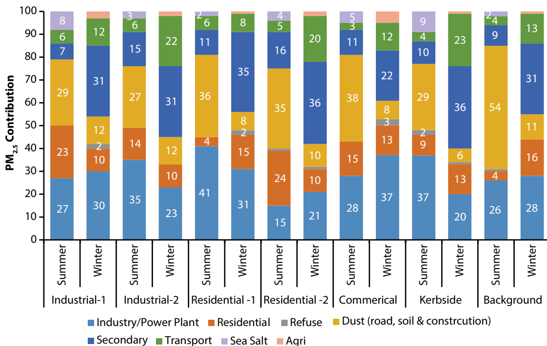
FIGURE 4.2: Estimated contributions of different sources to ambient PM_{2.5} at different monitoring locations
