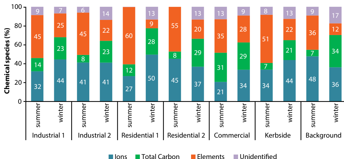
FIGURE 3.1: Seasonal variation in chemical characterization of ambient PM 10 at seven monitoring locations
