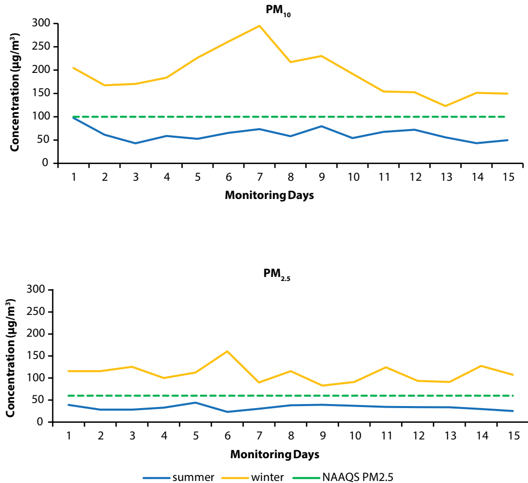
FIGURE 2.9: Variations of PM_{10} and PM_{2.5} concentrations for both seasons at industrial location - 2
