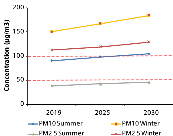
FIGURE 8.2: Winter and summer time projected particulate matter concentration in Surat city during the year 2019, 2025 and 2030 in BAU scenario.
