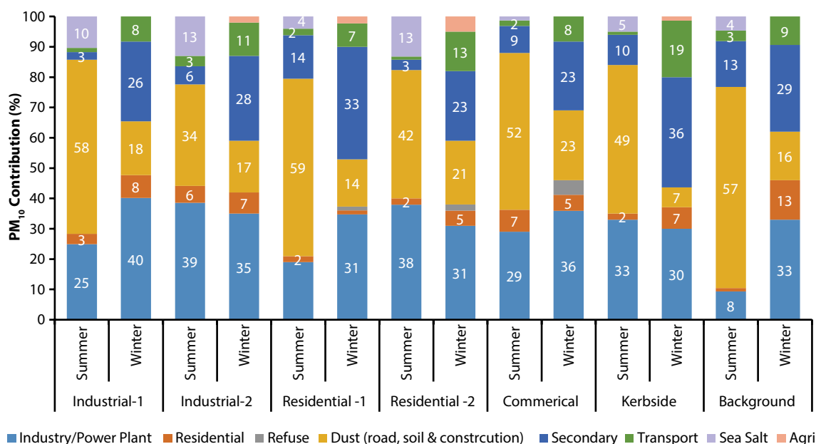
FIGURE 4.1: Estimated contributions of different sources to ambient PM_{10} at different monitoring locations during the two season
