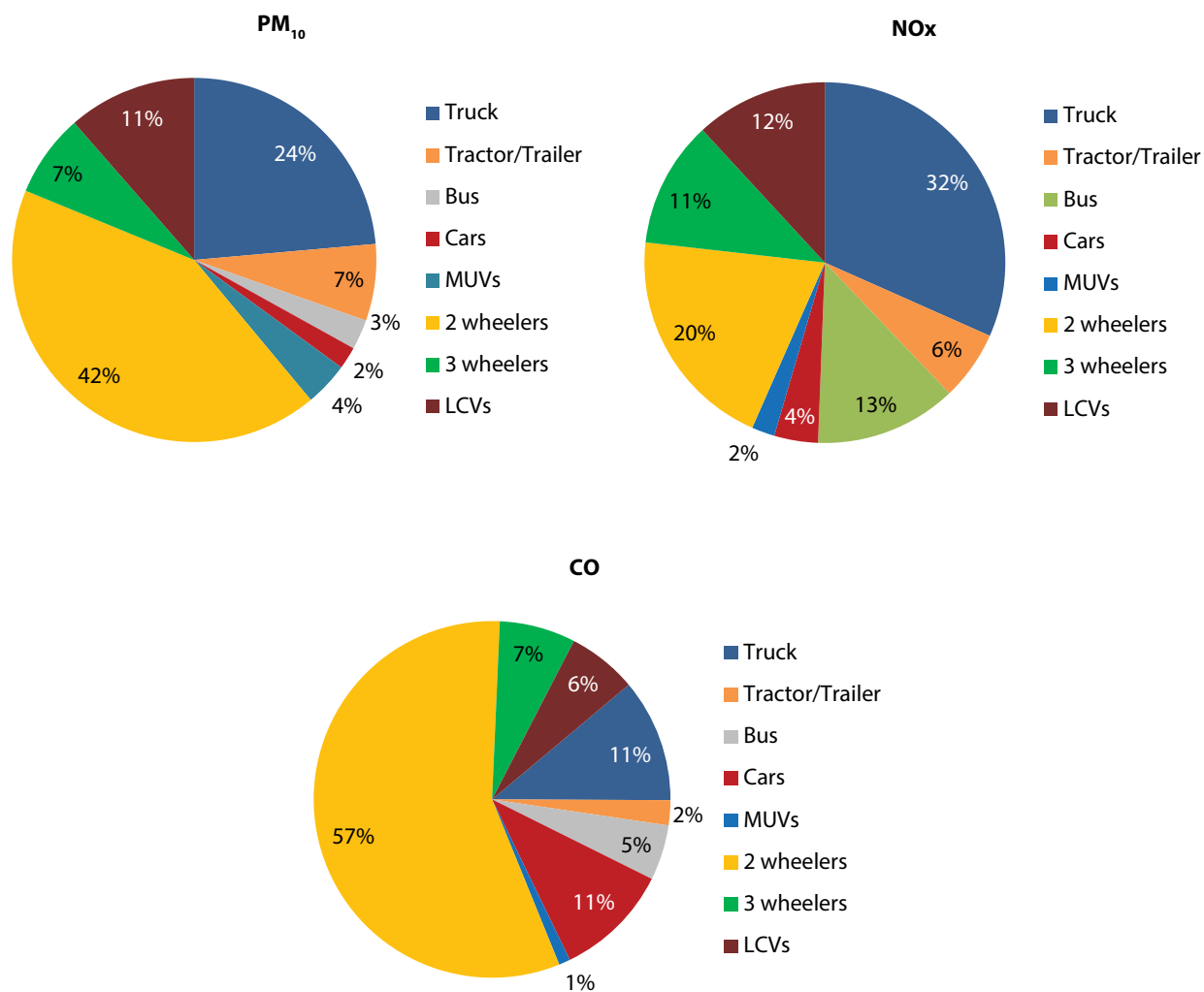
FIGURE 5.9: Distribution of PM, NO x and CO emissions in Surat City
