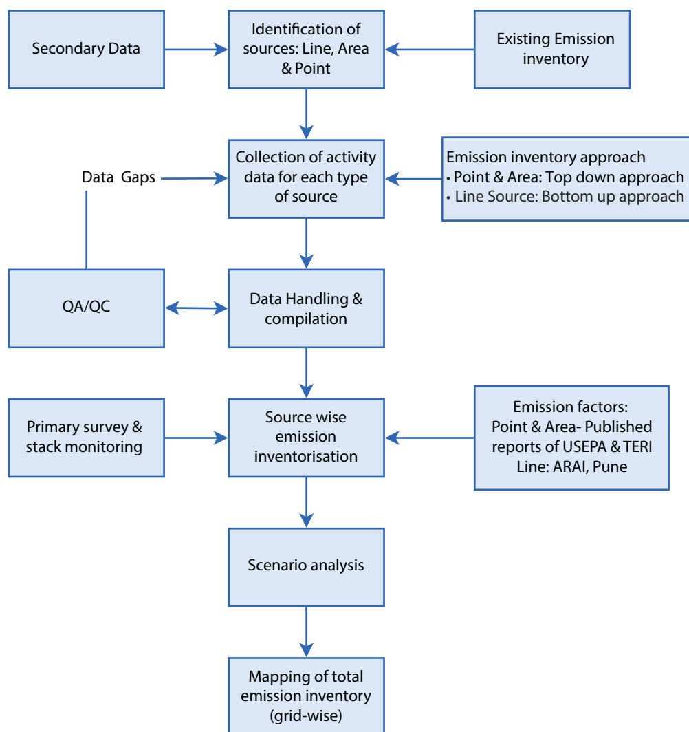
FIGURE 1.2: Overall approach for emission inventurisation of Surat city
