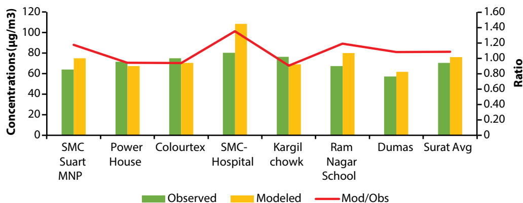
FIGURE 6.3: Simulated and observed concentrations ( \mu\text{g}/\text{m}^3 ) in across Surat.
