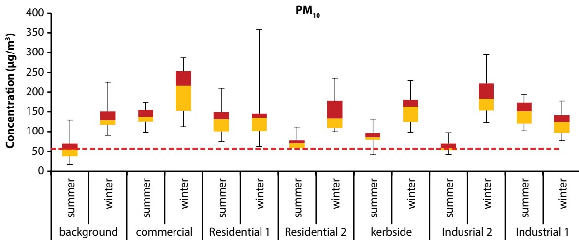
FIGURE 2.11: PM 10 concentration at different monitoring locations in Surat during winter and summer season
