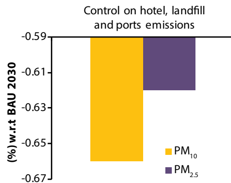
FIGURE 8.7: PM_{10} and PM_{2.5} emission reduction potential of strategy in others sector in the year 2030.
