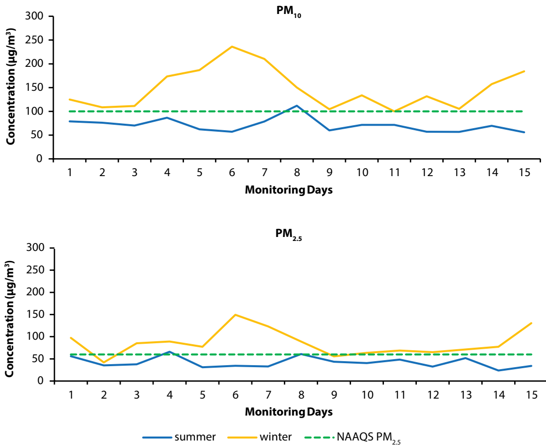
FIGURE 2.6: Variations of PM_{10} and PM_{2.5} concentrations for both seasons at residential location 2
