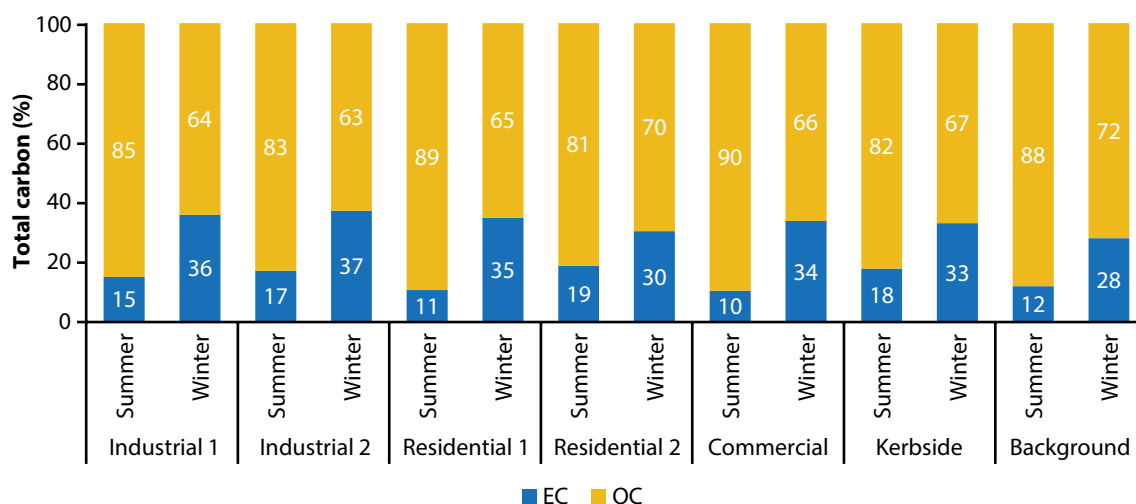
FIGURE 3.8: Seasonal variation of different fractions of carbon in ambient PM_{2.5} at different monitoring locations
