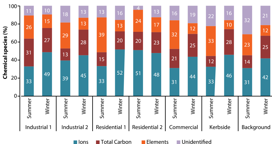
FIGURE 3.5: Seasonal variations in chemical characterization of ambient PM 2.5 at different monitoring locations
