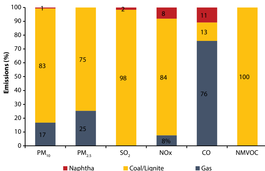
FIGURE 5.15: Percentage shares of pollutants emitted from different fuel based thermal power plants in Surat
