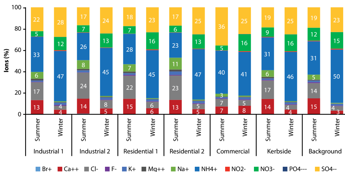
FIGURE 3.3: Seasonal variation in ionic composition of ambient PM_{10} at different monitoring locations in Surat
