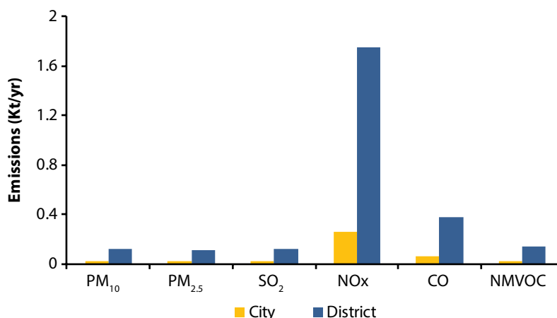
FIGURE 5.17: City and district level emissions from diesel generators
