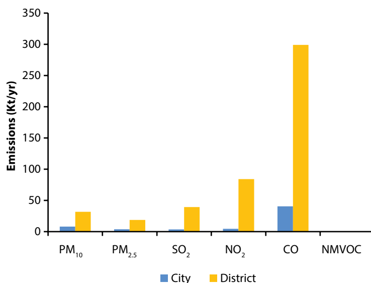
FIGURE 5.2: Emission from industries in Surat situated in district and city
