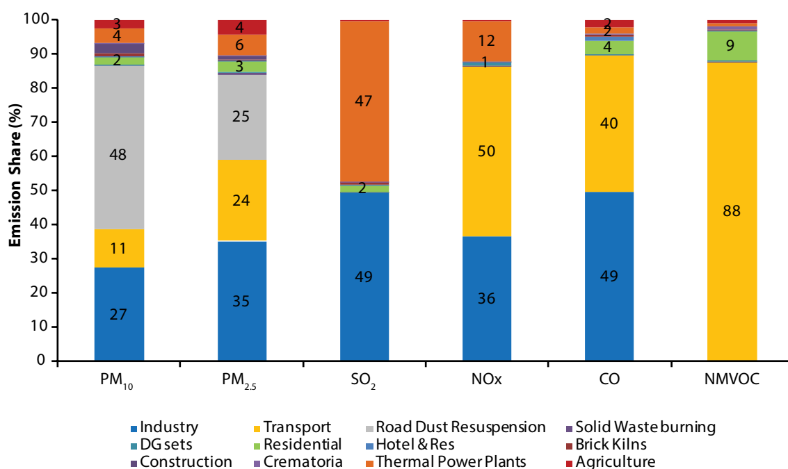
FIGURE 5.20: Percentage emissions share of various sources in Surat District
