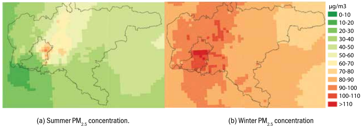
FIGURE 6.2: Spatial \text{PM}_{2.5} concentration ( \mu\text{g}/\text{m}^3 ) in summer and winter seasons
