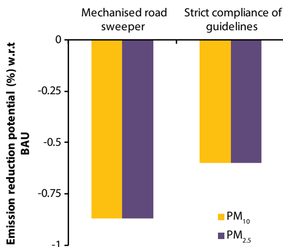
FIGURE 8.6: Emission reduction potential of the strategies with respect to sectoral emissions in BAU 2030
