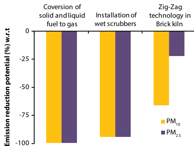
FIGURE 8.5: Emission reduction potential of various strategies w.r.t 2030
