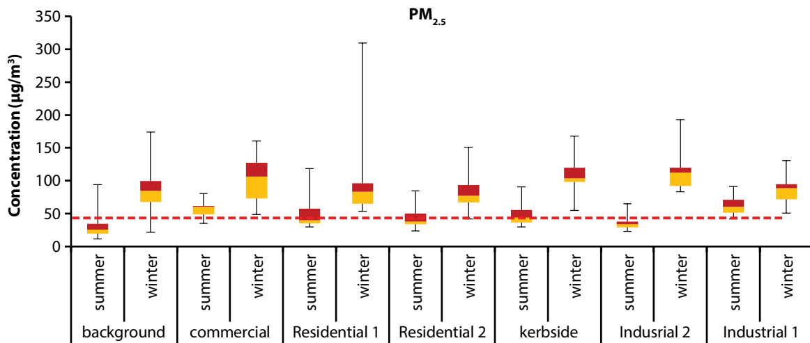
FIGURE 2.12: PM 2.5 concentration at different monitoring locations in Surat during winter and summer season
