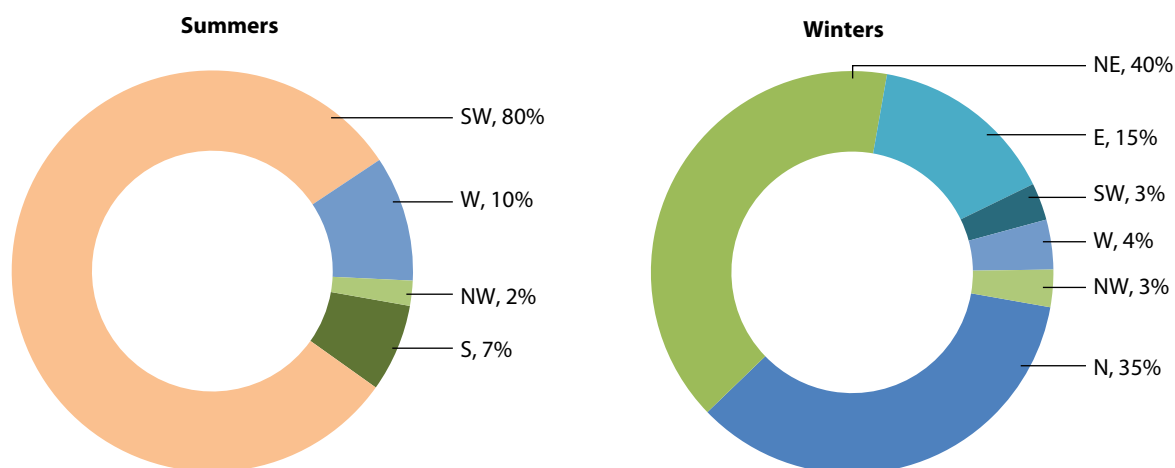
FIGURE 2.2: (b) Wind direction distribution at Surat in both summers & winters season
