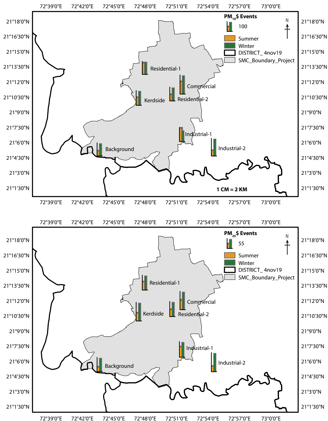
FIGURE 2.10: spatial distribution of PM_{10} and PM_{2.5} for both summer and winter season
