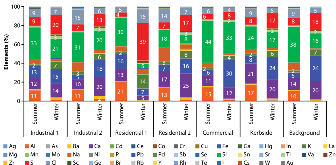
FIGURE 3.2: Seasonal variation in shares of various elements in ambient PM_{10} concentrations at seven monitoring locations in Surat
