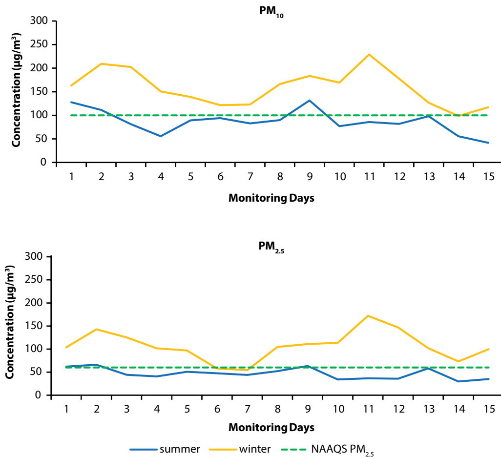
FIGURE 2.8: Variations of PM_{10} and PM_{2.5} concentrations for different seasons at industrial location 1
