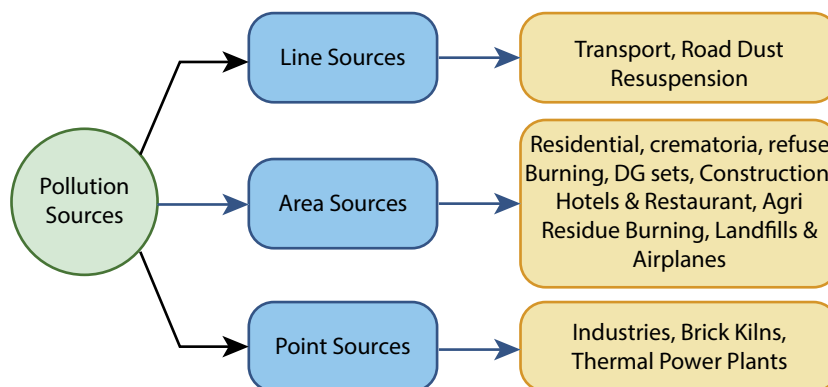
FIGURE 5.1– Different pollution sources inventorised in this study for Surat
