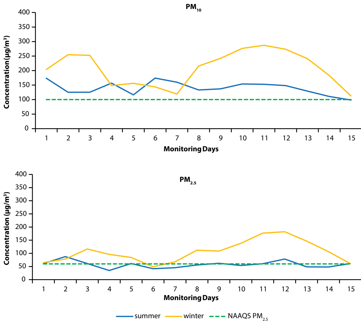
FIGURE 2.4: Trend of PM_{10} and PM_{2.5} levels for different seasons at commercial location
