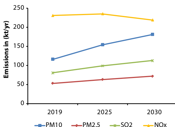
FIGURE 8.1: Emissions of PM_{10} , PM_{2.5} , SO_2 , and NO_x during 2019, 2025 and 2030 for Surat city in BAU scenario
