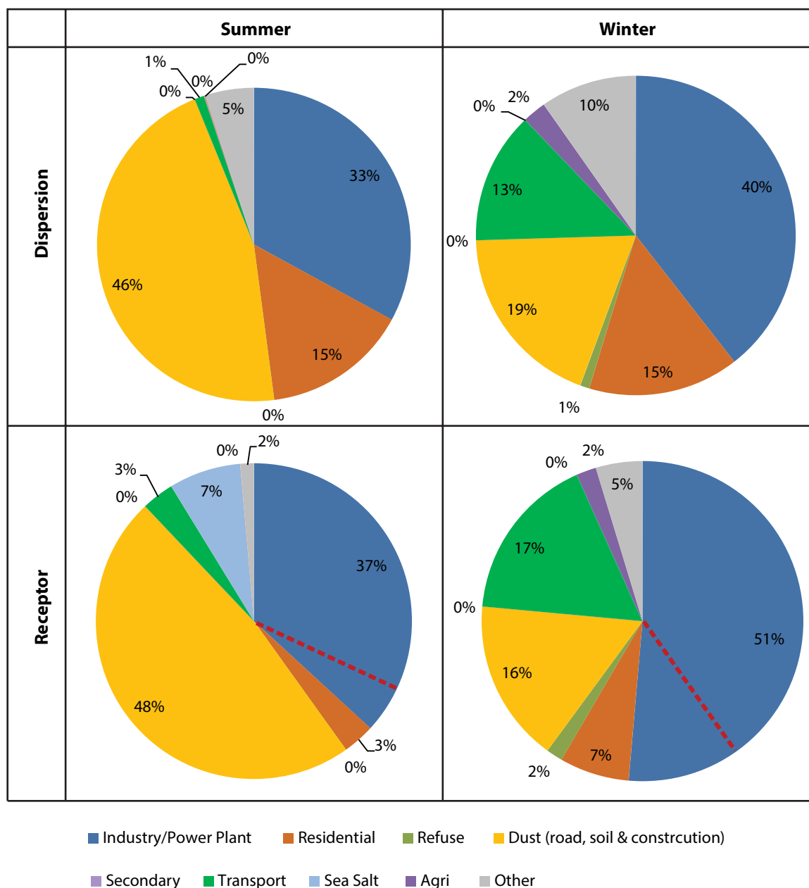
FIGURE 7.2: Comparative analysis of Receptor Modelling and Dispersion modelling estimates of sources contributions towards ambient PM_{10} concentrations in Surat
