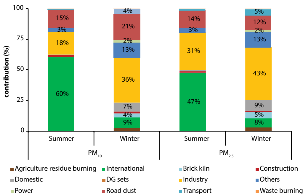
FIGURE 8.3: Sectoral contribution in PM_{10} and PM_{2.5} concentration of Surat city in summer and winter season during the year 2030.
