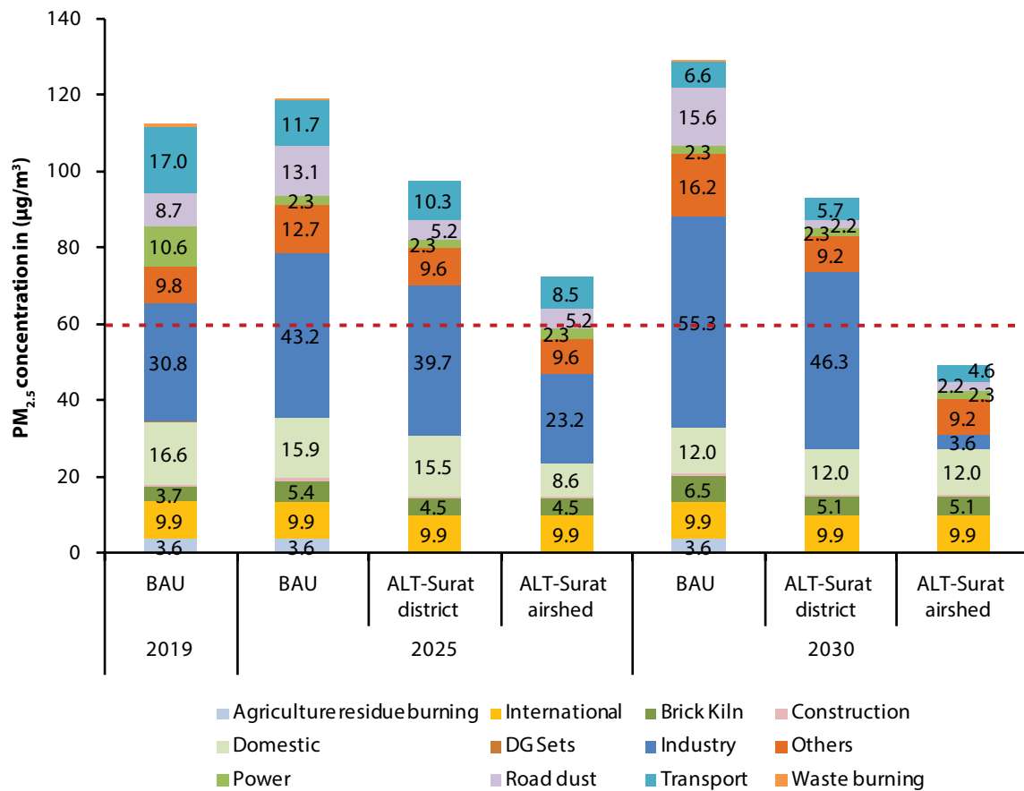
FIGURE 8.9: Winter season PM 2.5 concentration in different scenario in the Surat city
