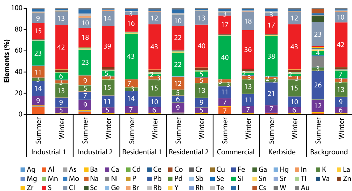
FIGURE 3.6: Seasonal variation in speciation of elements in ambient PM_{2.5} at different monitoring locations in Surat
