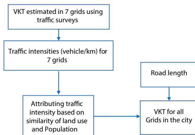
FIGURE 5.8: Method used for emission assessment of transport sector in the study area
