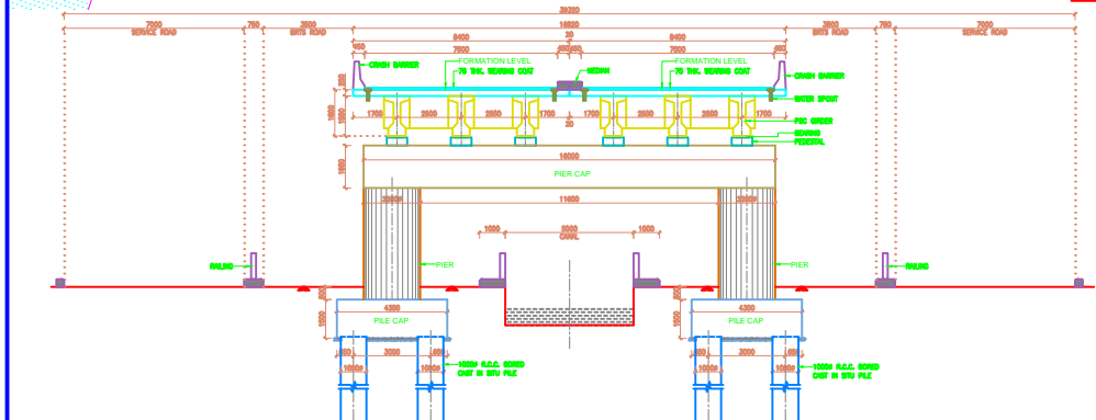
CROSS SECTION FOR 30.00m SPAN & 25.00m SPAN SCALE 1/25
