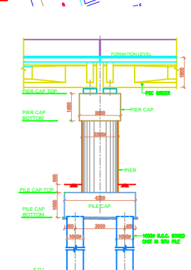
LONGITUDINAL SECTION FOR 30.00m SPAN & 25.00m SPAN SCALE 1/25
