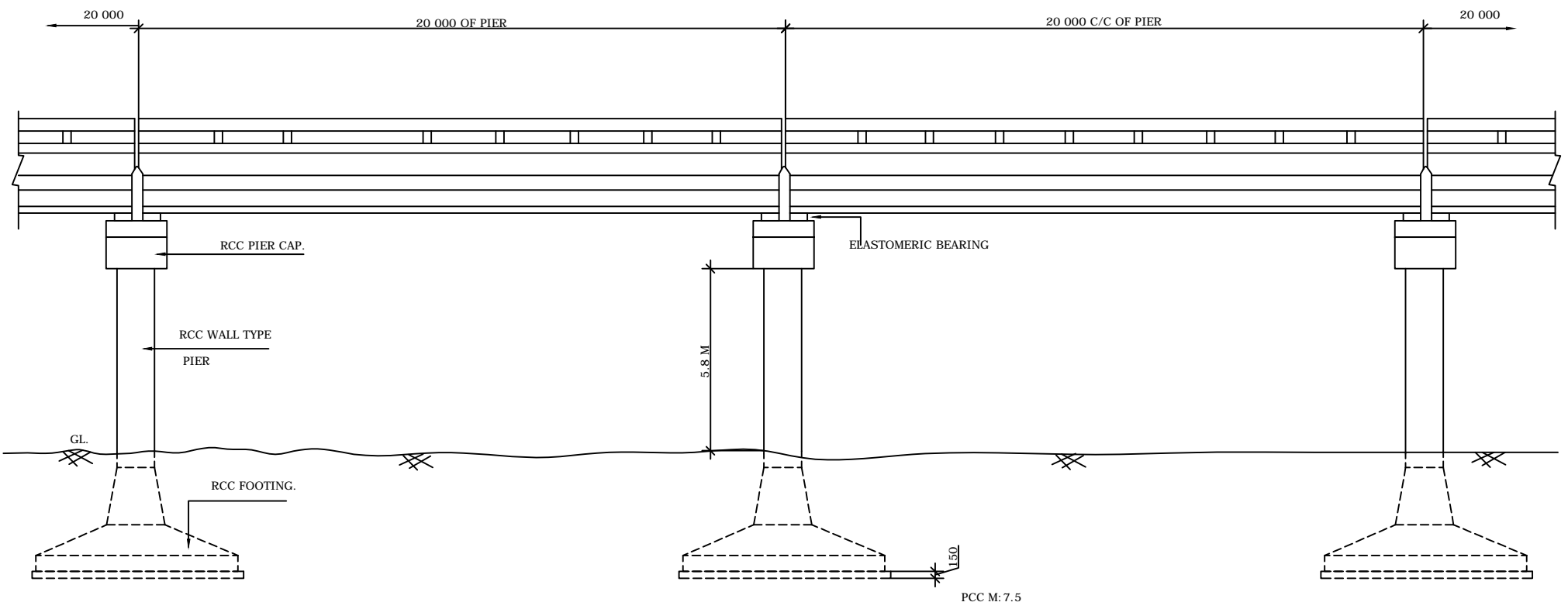
SECTIONAL ELEVATION
