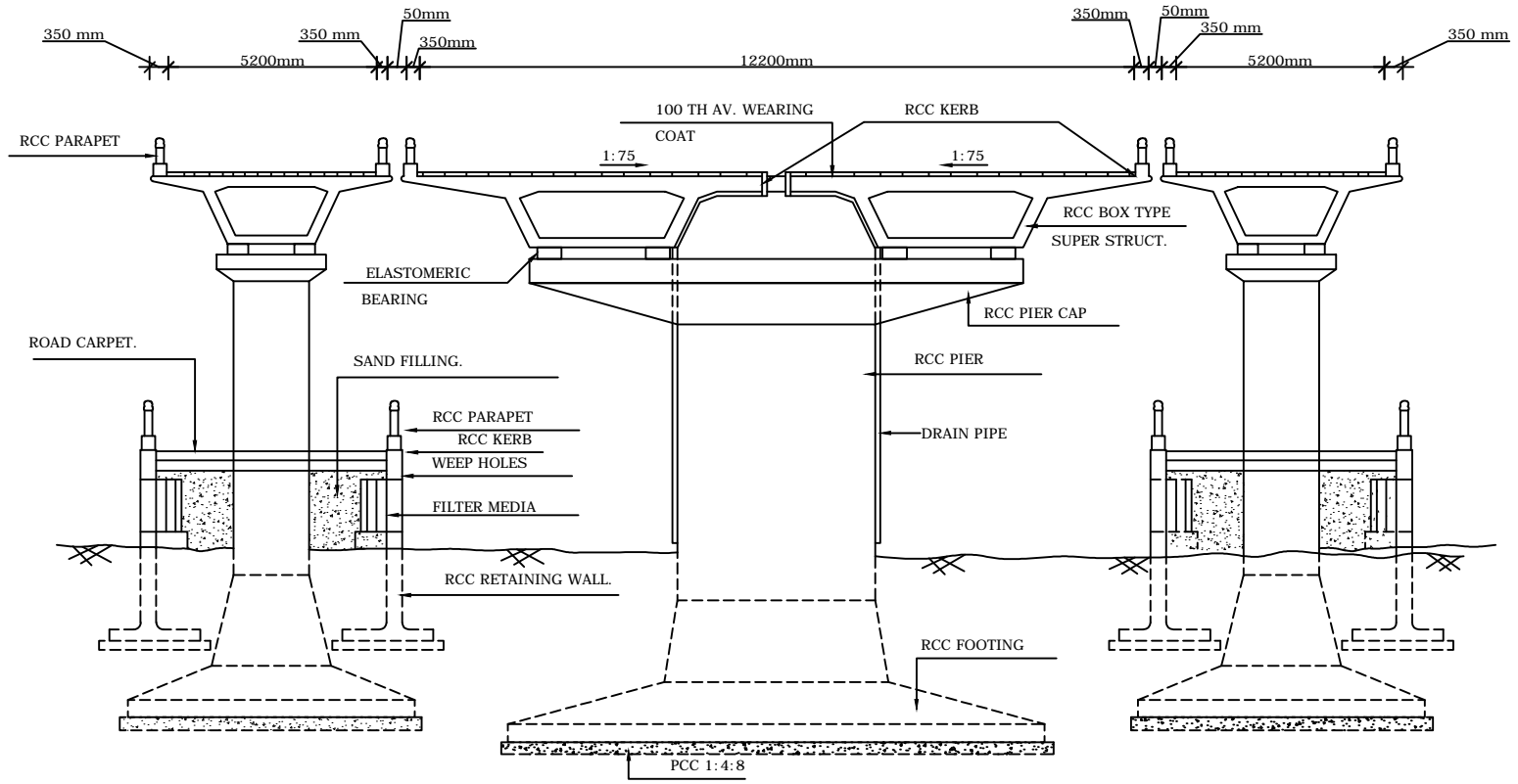
CROSS SECTION (NEAR RAMP)
