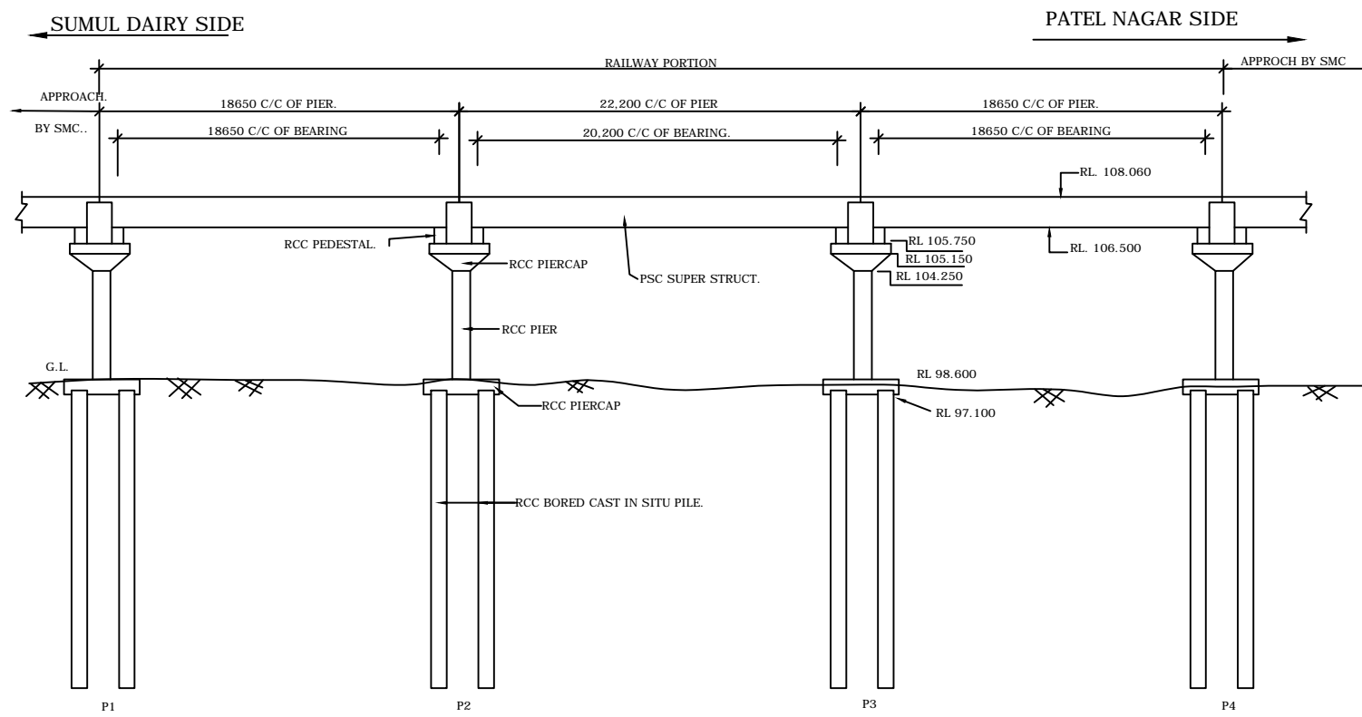
SECTIONAL ELEVATION
