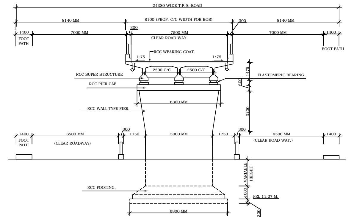
CROSS SECTION
