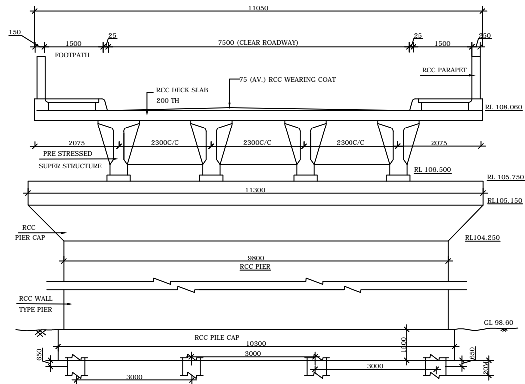
CROSS SECTION
